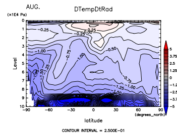
Figure 536: (\partial T/\partial t)_{SW+LW} at Aug. by DCPAM
