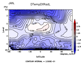
Figure 841: (\partial T / \partial t)_{LW} at Jan. by DCPAM
