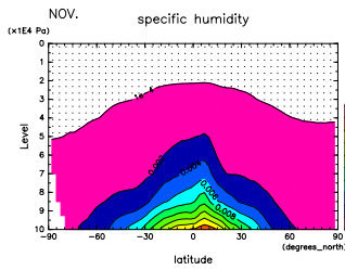
Figure 427: q at Nov. by DCPAM
