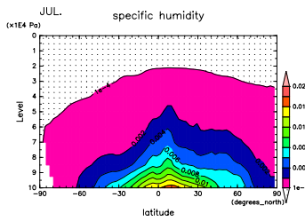
Figure 415: q at Jul. by DCPAM
