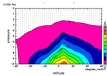
Figure 419: q at Aug. by NCEP
