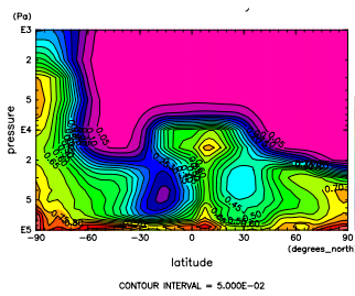
Figure 776: RH at Jul. by NCEP
