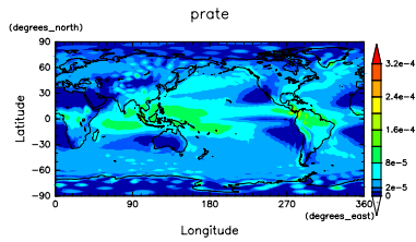
Figure 14: Annual mean Rain by DC-PAM
