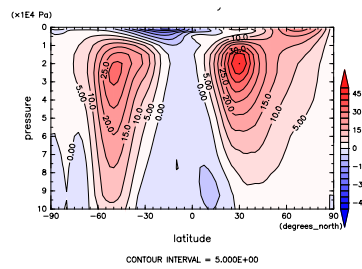
Figure 221: U at Feb. by NCEP
