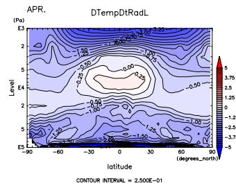
Figure 844: (\partial T/\partial t)_{LW} at Apr. by DCPAM
