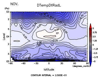
Figure 851: (\partial T/\partial t)_{LT} at Nov. by DCPAM Figure 852: (\partial T/\partial t)_{LT} at Dec. by DCPAM
