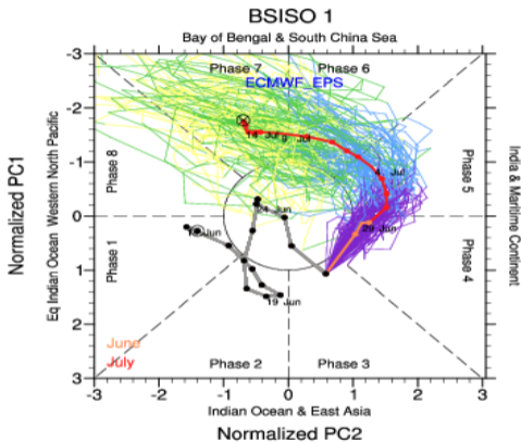
BSISO Forecast for 28-June-2026 to 17-July-2026
