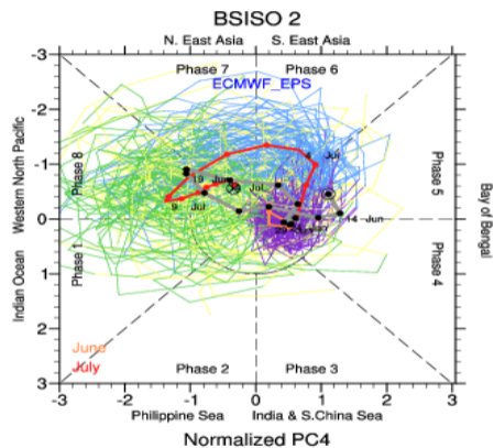
BSISO Forecast for 28-June-2026 to 17-July-2026
