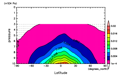
Figure 424: q at Oct. by DCPAM
