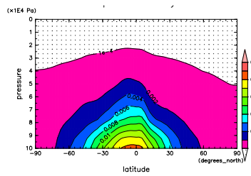
Figure 398: q at Jan. by NCEP
