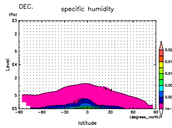
Figure 754: q at Dec. by DCPAM
