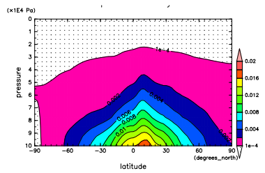
Figure 422: q at Sep. by NCEP
