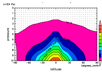
Figure 407: q at Apr. by NCEP
