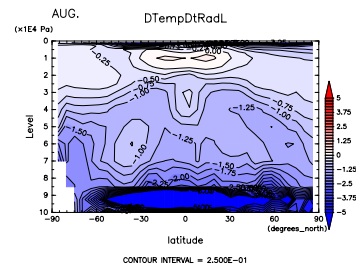
Figure 524: (\partial T/\partial t)_{LW} at Aug. by DCPAM
