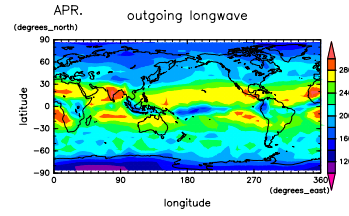
Figure 127: OLR at Mar. by DCPAM Figure 130: OLR at Apr. by DCPAM
