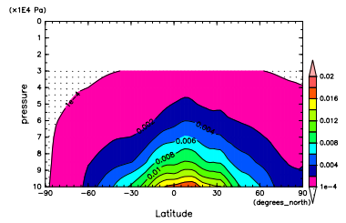
Figure 421: q at Sep. by DCPAM
