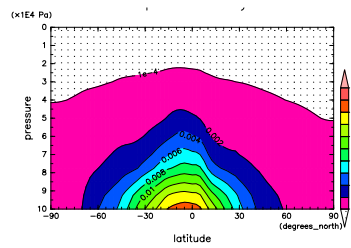
Figure 401: q at Feb. by NCEP
