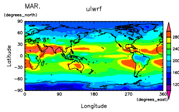
Figure 127: OLR at Mar. by DCPAM Figure 130: OLR at Apr. by DCPAM
