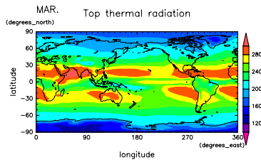
Figure 128: OLR at Mar. by NCEP Figure 131: OLR at Apr. by NCEP
