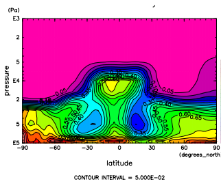
Figure 764: RH at Mar. by NCEP
