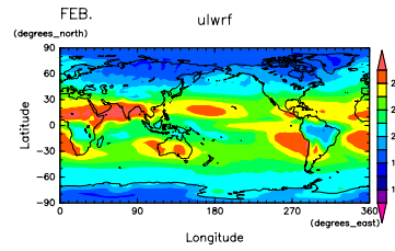
Figure 124: OLR at Feb. by DCPAM
