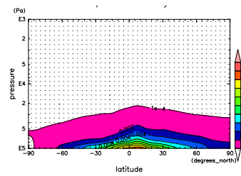
Figure 737: q at Jun. by NCEP
