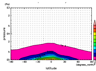
Figure 755: q at Dec. by NCEP
