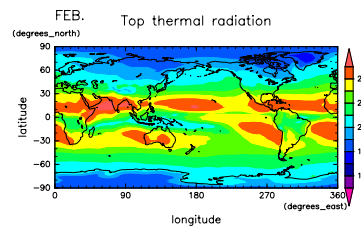
Figure 125: OLR at Feb. by NCEP
