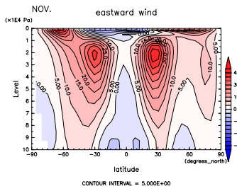
Figure 247: U at Nov. by DCPAM
