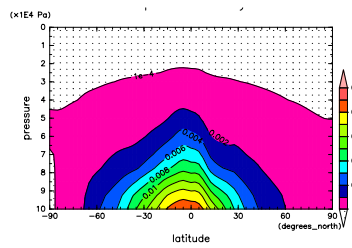
Figure 404: q at Mar. by NCEP
