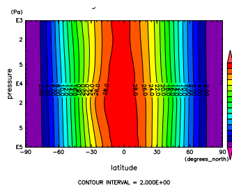
Figure 596: ANGMOM at Jul. by NCEP
