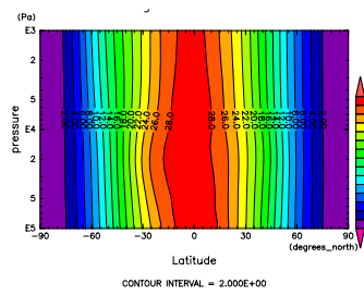
Figure 598: ANGMOM at Aug. by DCPAM
