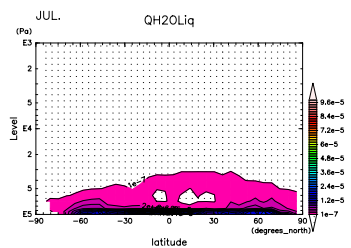
Figure 799: q_l at Jul. by DCPAM
