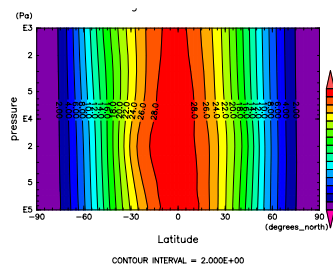
Figure 595: ANGMOM at Jul. by DCPAM
