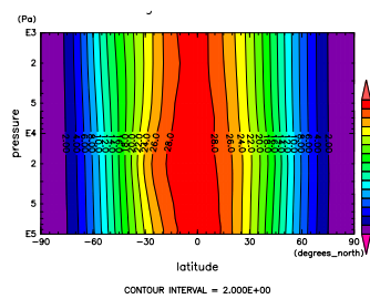
Figure 599: ANGMOM at Aug. by NCEP
